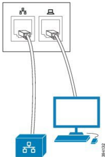
Figure 3: Phone Network Connections
