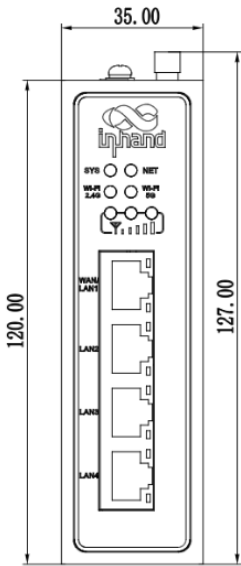
Interface Diagram
